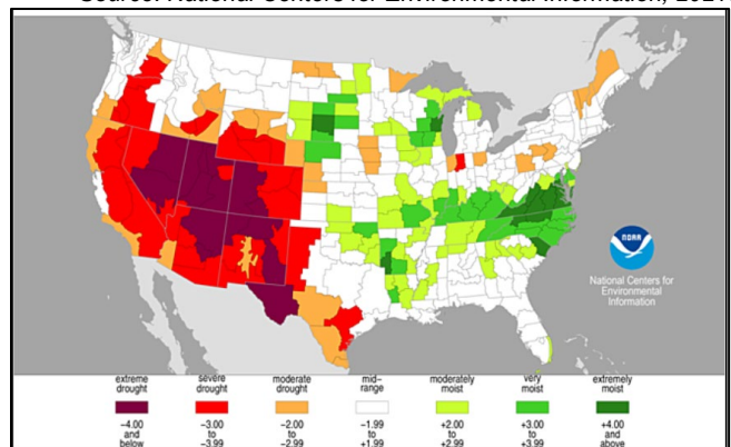
Figure 8-4. Palmer Hydrological Drought Index (January 2021)
